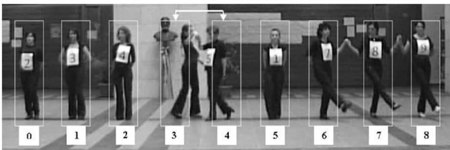
Fig. 2. Bubble-sort dance-performance.
