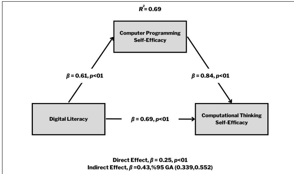
Figure 2. Structural Equation Model Analysis Results
